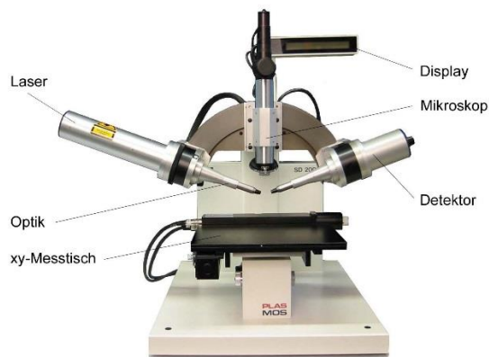
Ellipsometer
