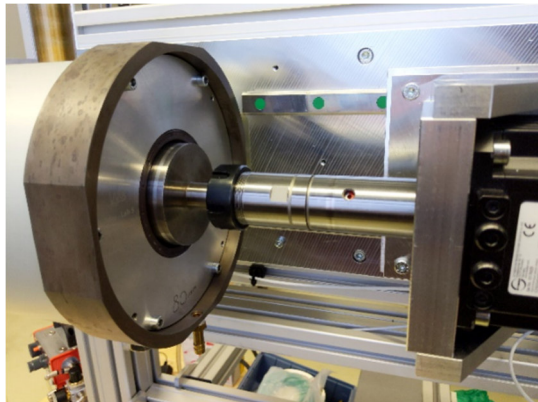
Water test bench (Test chamber and drive unit)
